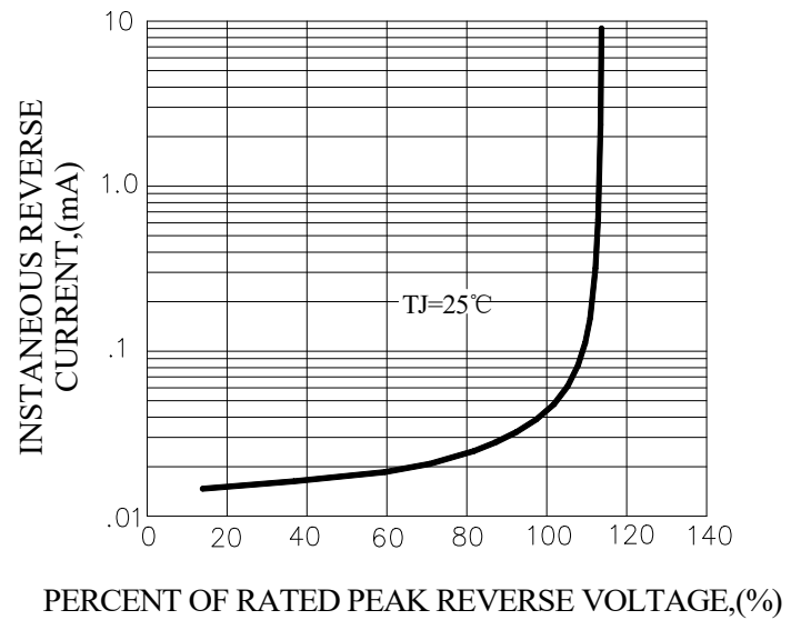
FIG.4-TYPICAL REVERSE CHARACTERISTICS
